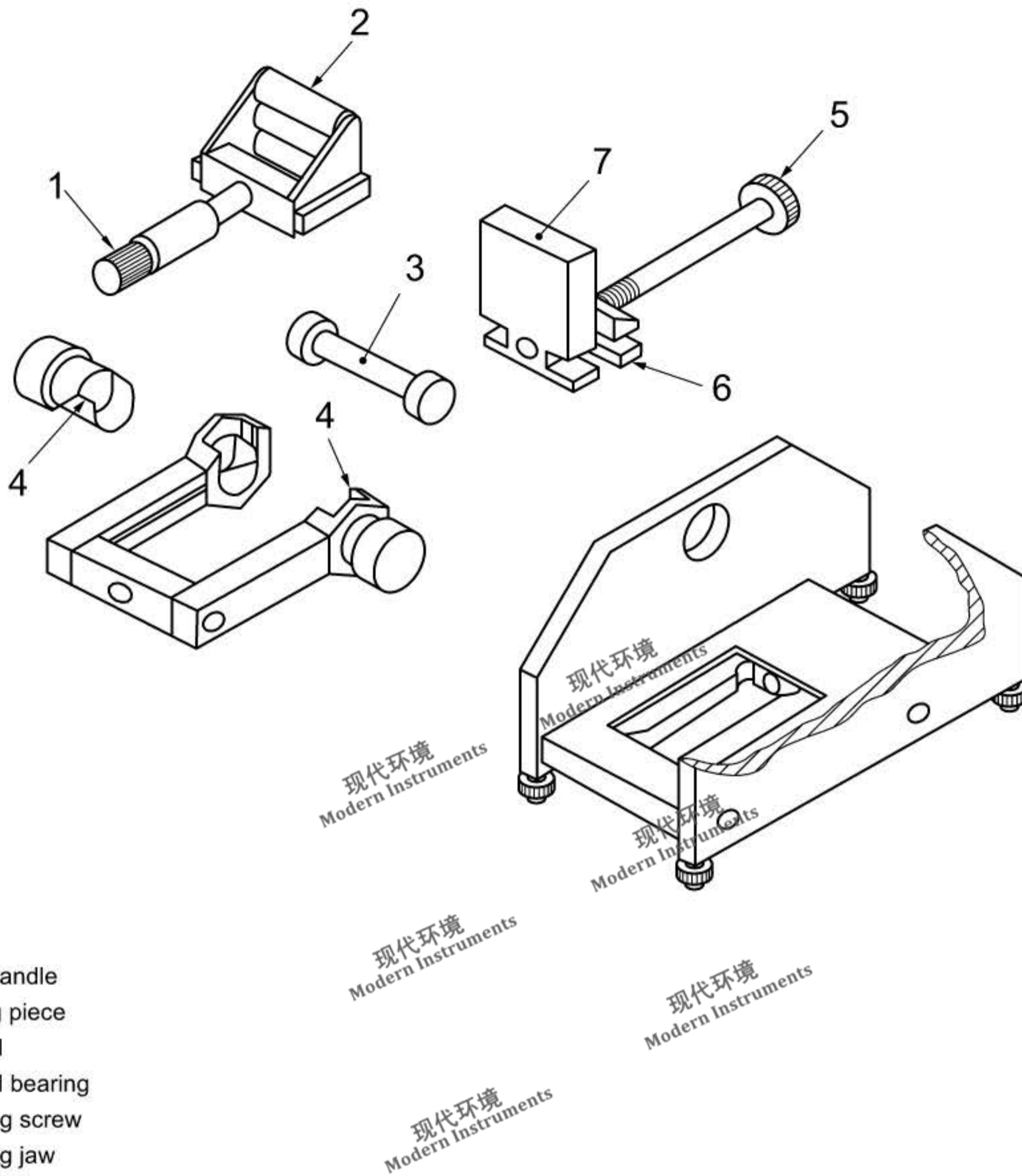
Figure 4 — Exploded diagram of the tester shown in Figure 3
