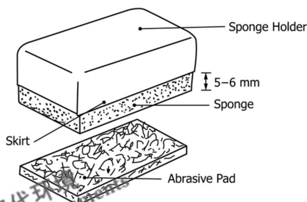
FIG. 2 Abrasion Boat Components
