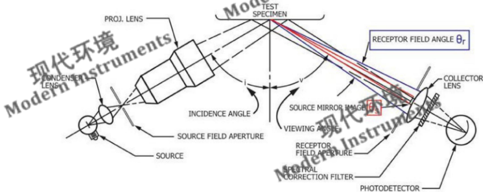
FIG. 2 Diagram of Converging-Beam Glossmeter Showing Apertures and Source Mirror-Image Position
