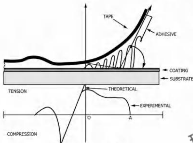
FIG. X1.1 Peel Profile (6)
