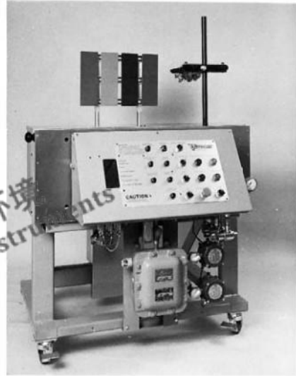
(b) Fixed Panel, Traveling Gun Machine
