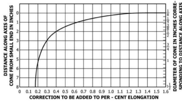
FIG. 3 Correction for Thickness of Film
