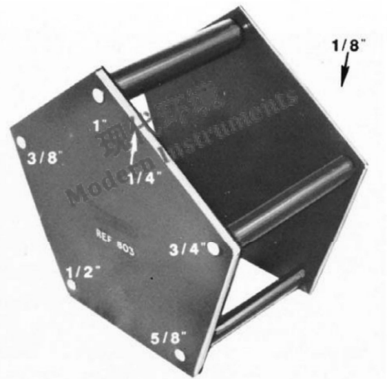
FIG. 4 An Illustration of a Cylindrical Mandrel Test Apparatus
