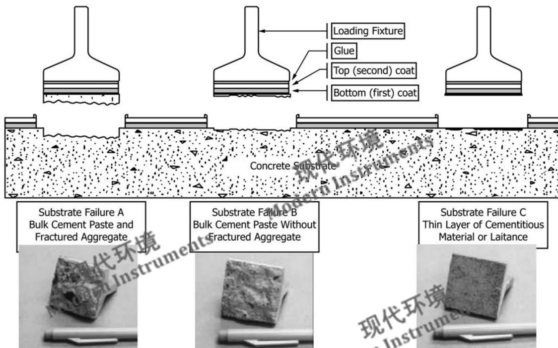
FIG. 3 Substrate Failure Classification
