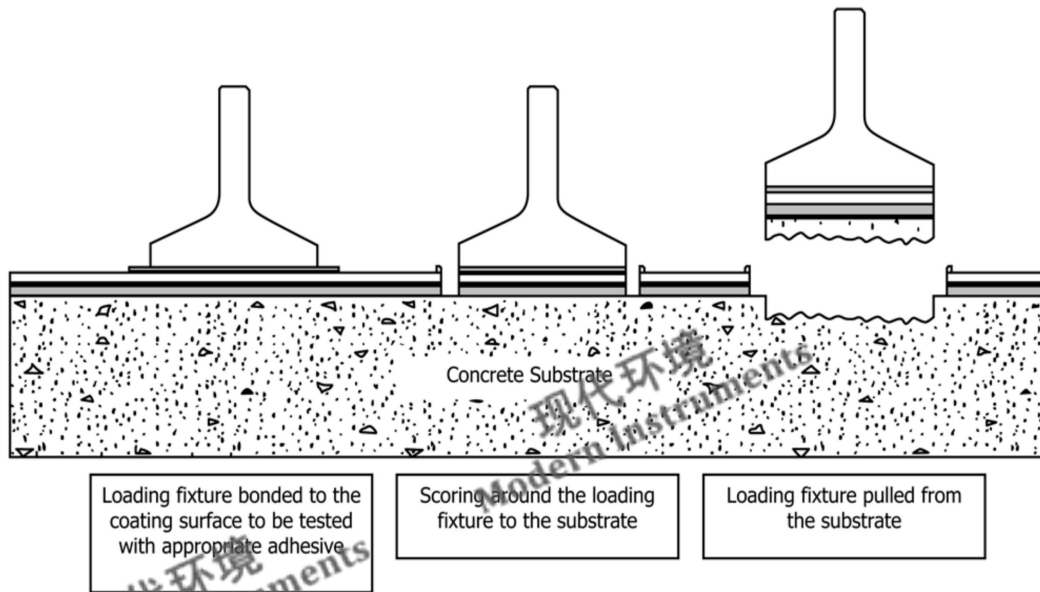
FIG. 2 Scoring Around the Loading Fixture After Attachment of the Fixture (Square or Rectangular Fixtures)
